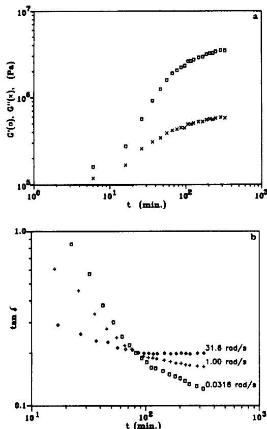
Figure 12. Evolution of (a) mechanical dynamic moduli at 1 rad/s and (b) the loss tangent at the indicated frequencies during crystallization of PP(25) at 40 °C after rapidly cooled from 100 °C. ( \square ) G' ; ( \times ) G'' .
