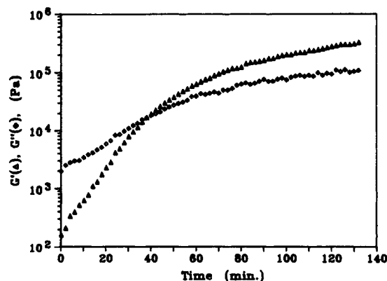
Figure 11. Dynamic moduli ( \omega = 1 rad/s) of PP(50) during isothermal crystallization at 60 °C. The sample was first heated to 100 °C and then rapidly cooled to 60 °C.
