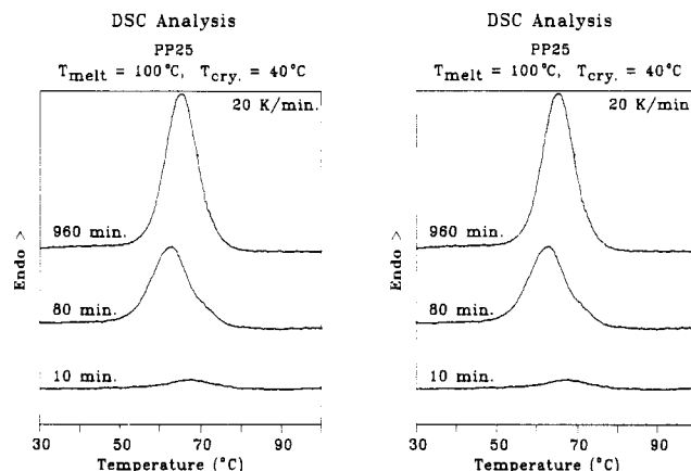
Figure 14. DSC variation with time of isothermal crystallization for (a) PP(25) and (b) PP(50).
