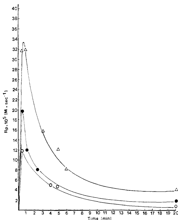
Figure 2. R_p versus time plots of the data in Figure 1. polymerization yield ( Y ). The intercept at Y = 0 gives the initial and maximum concentration of [\text{Ti-P}] , which is taken to be the initial concentration of the active species, [\text{C}^*]_0 . The values of [\text{C}^*]_0 were found to be 3.7, 4.25, and 3.7% of 3 for T_p at -20 , 0 , and +25^\circ\text{C} , respectively. The value of k_p was obtained from
