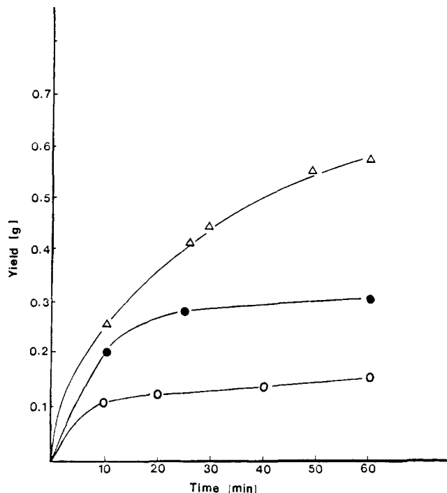
Figure 1. Yield versus time of propylene polymerizations catalyzed by 1/MAO with [3] = 27 \mu\text{M} , [\text{Al}]/[\text{Ti}] = 2000 , 100 mL of toluene, p_{\text{C}_3\text{H}_6} = 1.7 \text{ atm} , and T_p at (O) +25^\circ\text{C} , (●) 0^\circ\text{C} , and (Δ) -20^\circ\text{C} .
